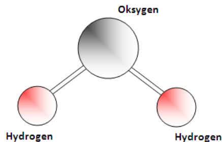
Vannmolekyl \text{H}_2\text{O}
